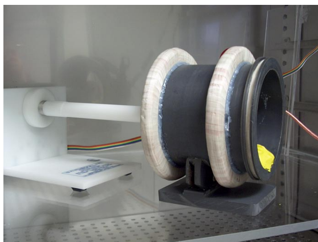
PEMF prototype device for initial studies.
